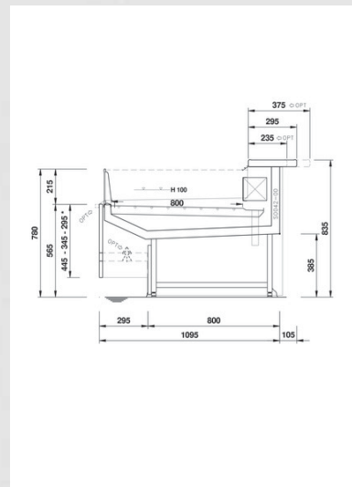
SELF-SERVICE COILED DECK
