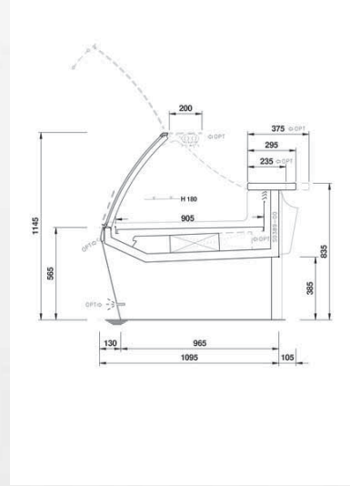
Ventilated with inclined understructure
