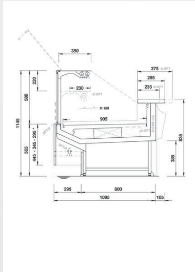
Ventilated with straight facing
